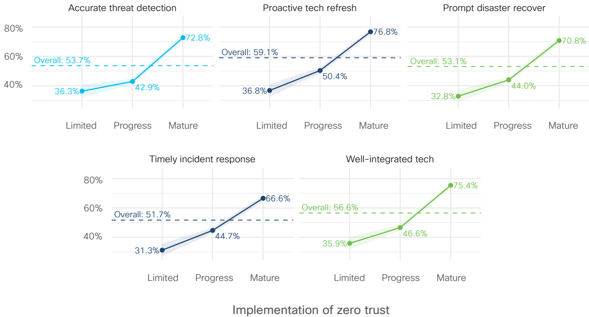
Figure 3: Zero trust adoption level and security practices
