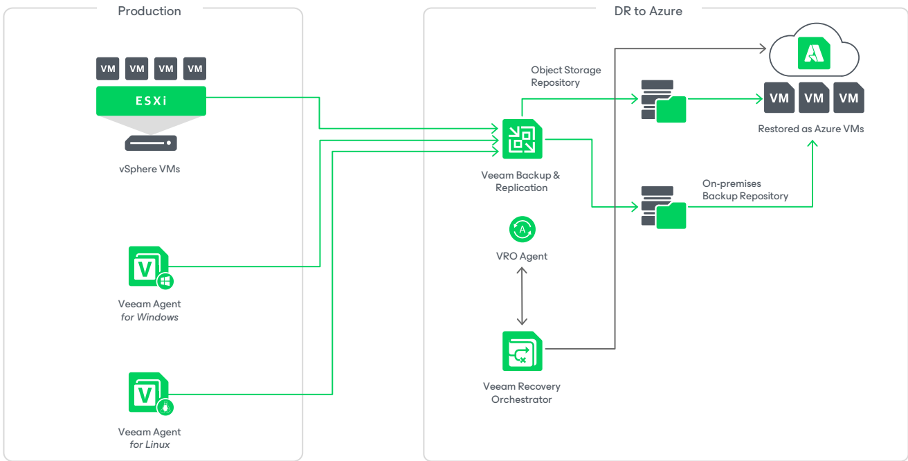
Figure 9 — Orchestrated recovery to Microsoft Azure
