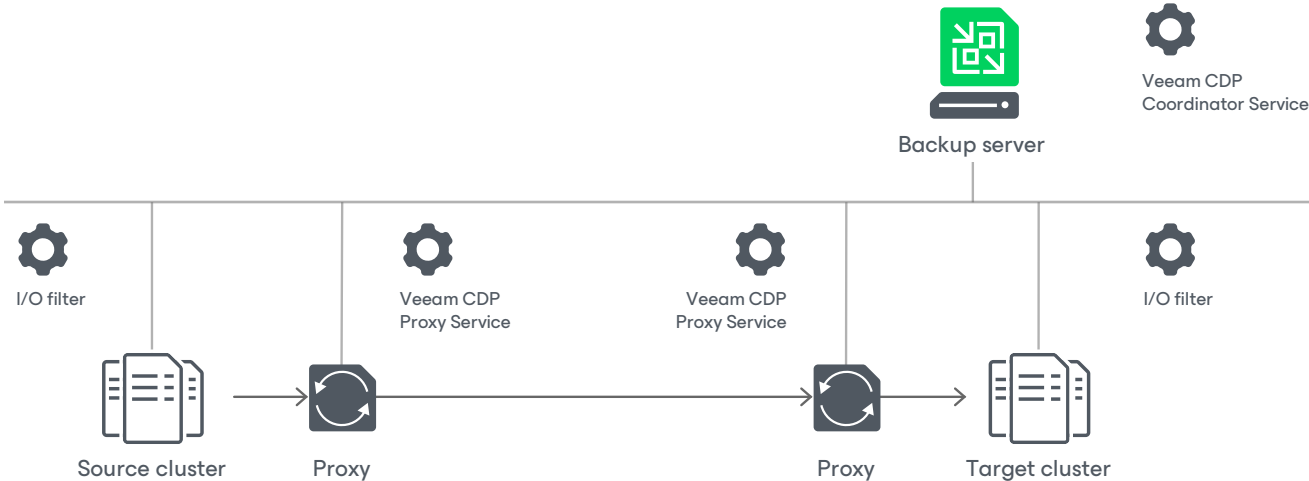
Figure 2 — Veeam CDP Architecture
